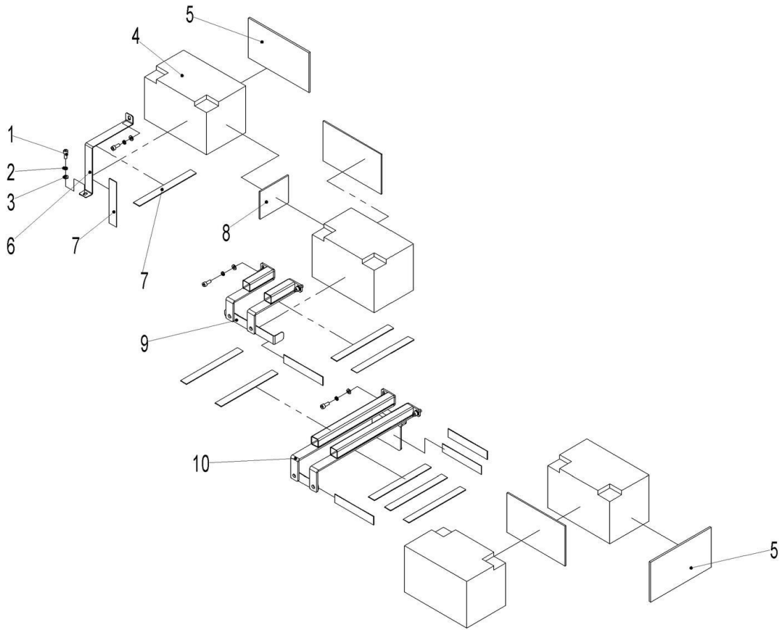
Fig. 15 Battery components
