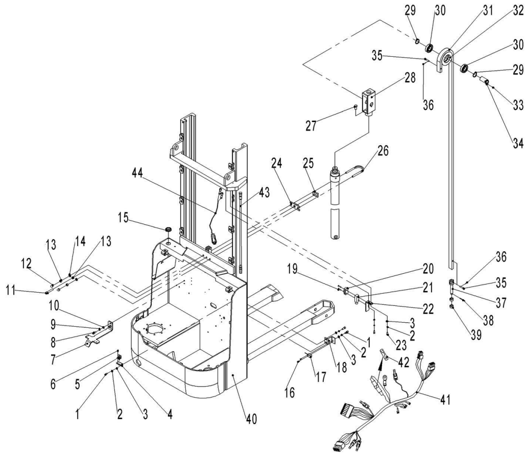
Fig. 17 Mast Assembly (One-stage mast)
